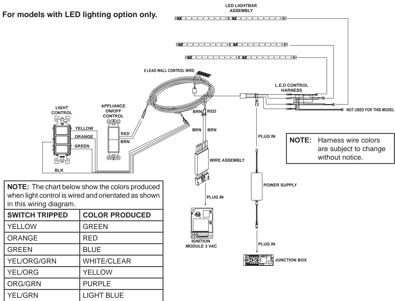
Figure 12.6 LED Wiring Diagram
