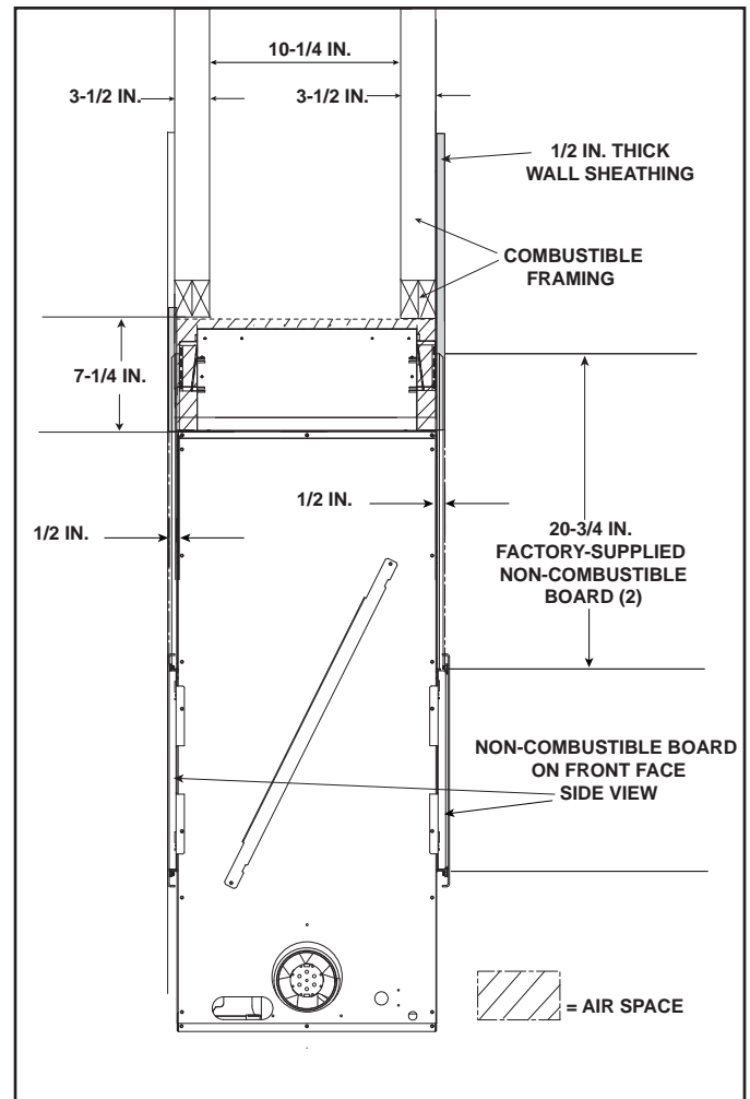
Figure 13.6 Framing and Framing Materials-RED40ST
