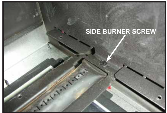
Figure 12.11. Side Burner Screw.
