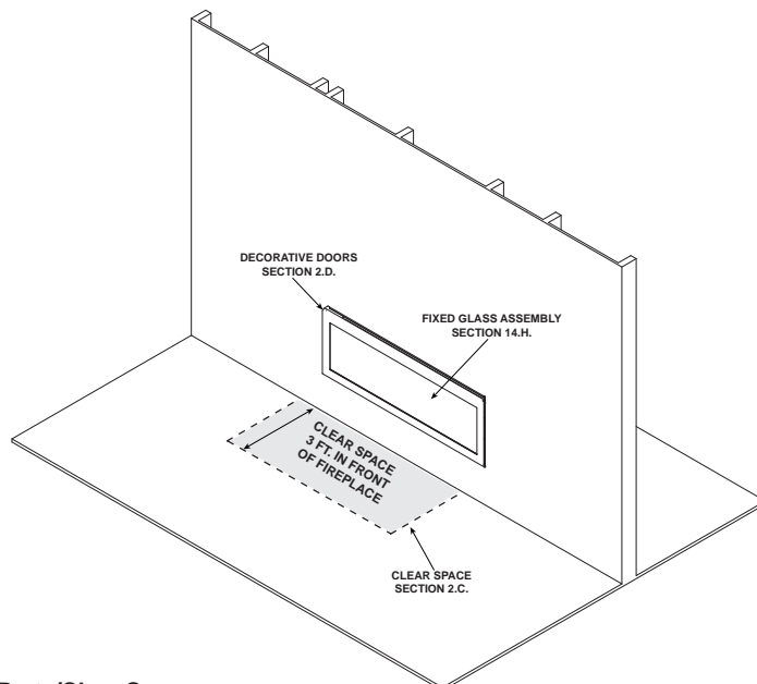
Figure 2.1 General Operating Parts/Clear Space.
