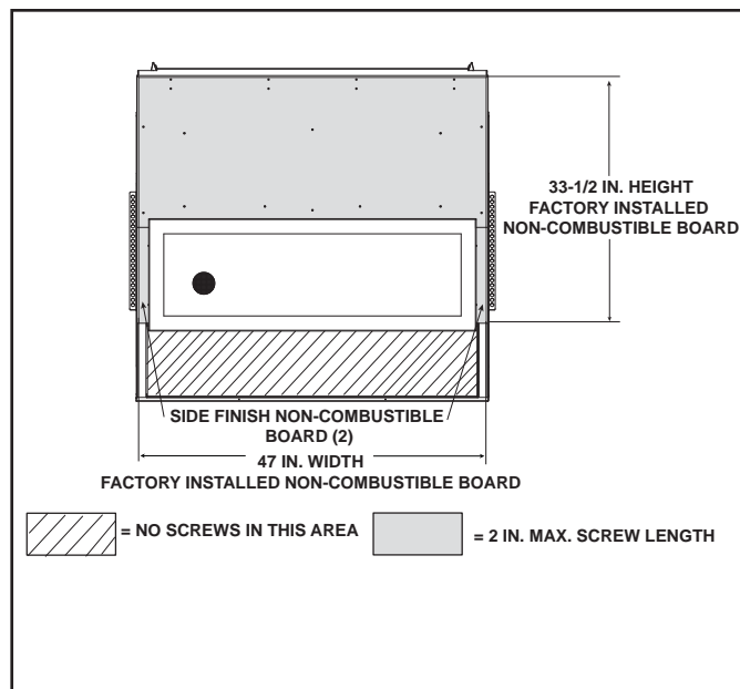
Figure 13.8 Non-Combustible Finish Material Diagram for 0-1 Inch Thick Overlap Fit Method
