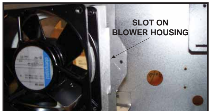
Figure 12.20. Blower Tab Inserted into Slot on Blower Housing
