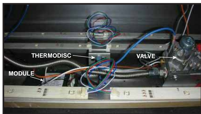
Figure 12.2. Valve Cavity
