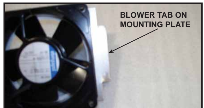
Figure 12.19. Blower Tab Toward Rear
