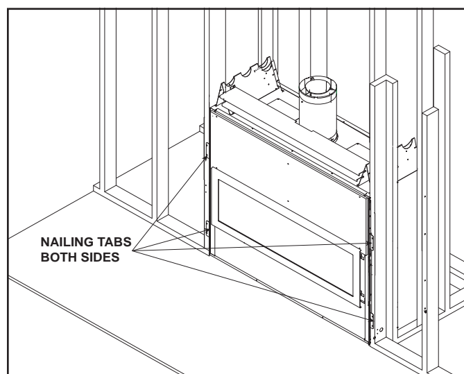
Figure 5.3 Nailing Tab Locations
