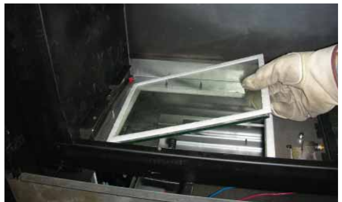
Figure 12.13. Removing Glass Pane Frame.
