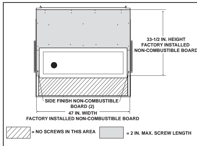
Figure 13.1 Finishing Details
