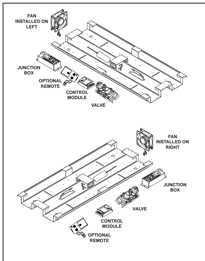
Figure 12.3. Controls Location Diagram
